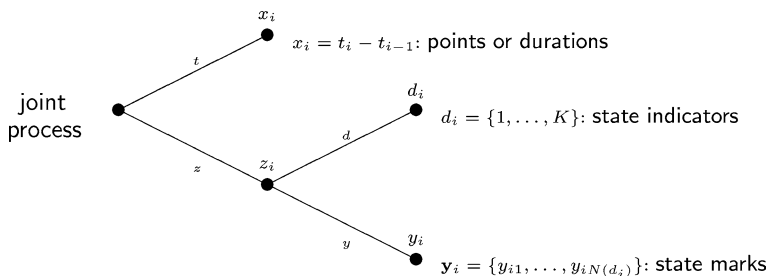
Decomposition of a Multi-State Marked Point Process
