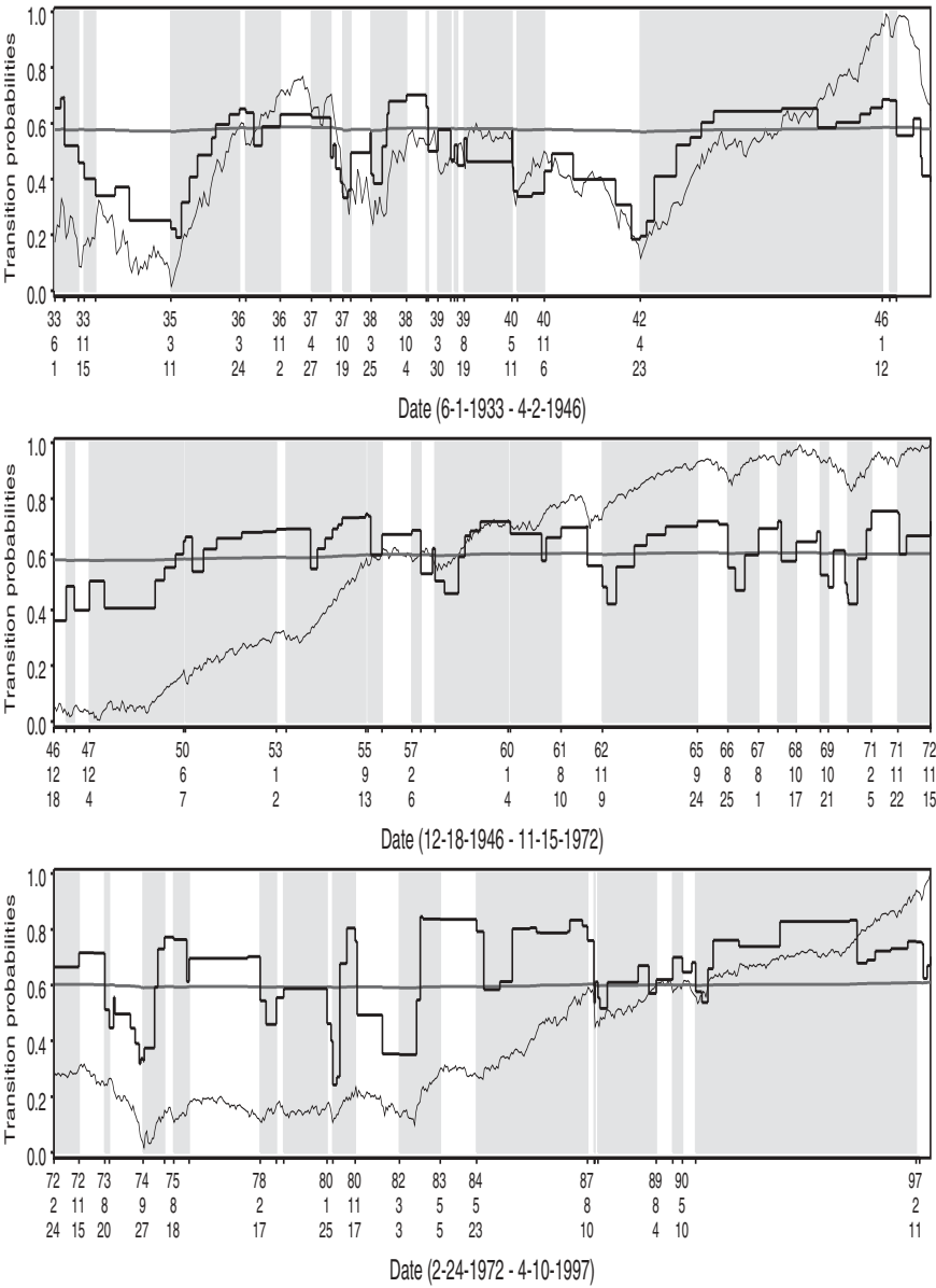
Figure 3. Transition probabilities (black line) from the MSMP-dyc model, for an 8% filter, plotted against log-prices (thin line). The nearly horizontal grey line tracks the unconditional transition probabilities. The shaded areas are periods of up durations
